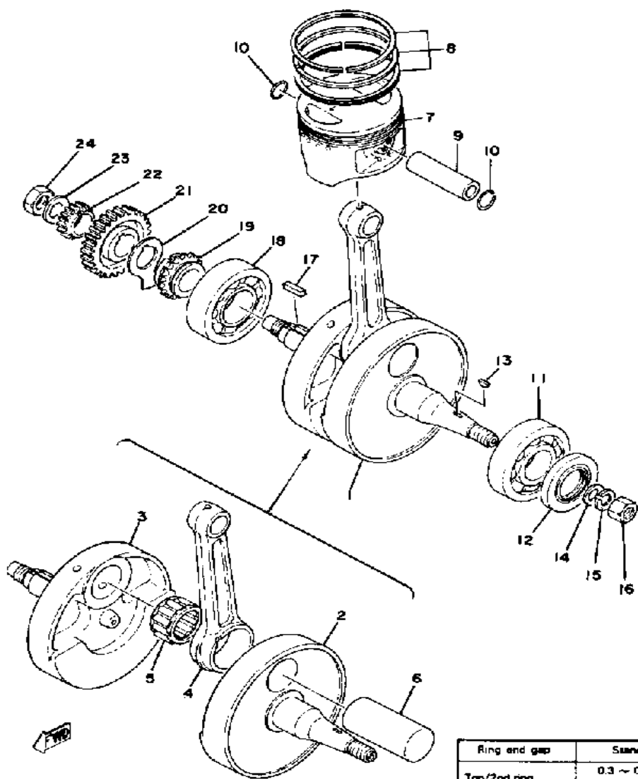
Crankshaft Specifications
